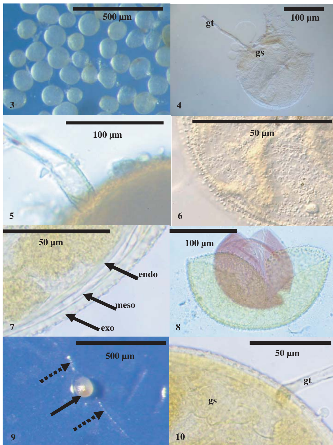
Figs 3–10. Gerdemannia scintillans . Fig. 3. Spores in water, freshly extracted from soil. Fig. 4. Spore (from the isotype) showing the lightly-pigmented germination shield (gs) and the germ tube (gt). Fig. 5. Spore (from the isotype) showing the attachment of the sub-stending hypha at the spore base and discolouration as the result of storage in 0.025 % sodium azide solution. Fig. 6. Spore surface showing ornamentation viewed with Nomarski differential interference contrast. Fig. 7. Wall structure of exospore ('exo'), mesospore ('meso') and endospore ('endo'). The mesospore can be seen adherent to the exospore (lower left), crossing over to the endospore (upper, right). Fig. 8. Melzer's reaction of the endospore; note the apparent difference in colour where the yellow-stained exospore is acting as a coloured filter; the true colour reaction can be seen only where the endospore is extruded from its encompassing wall components. Fig. 9. Spore germinating on a membrane filter; the lightly pigmented germination shield is indicated by a solid arrow, and the germination hyphae by dotted arrows. Fig. 10. Details of germination shield with crenulated edges (beneath gs) and germ tube (gt) (from the isotype).
