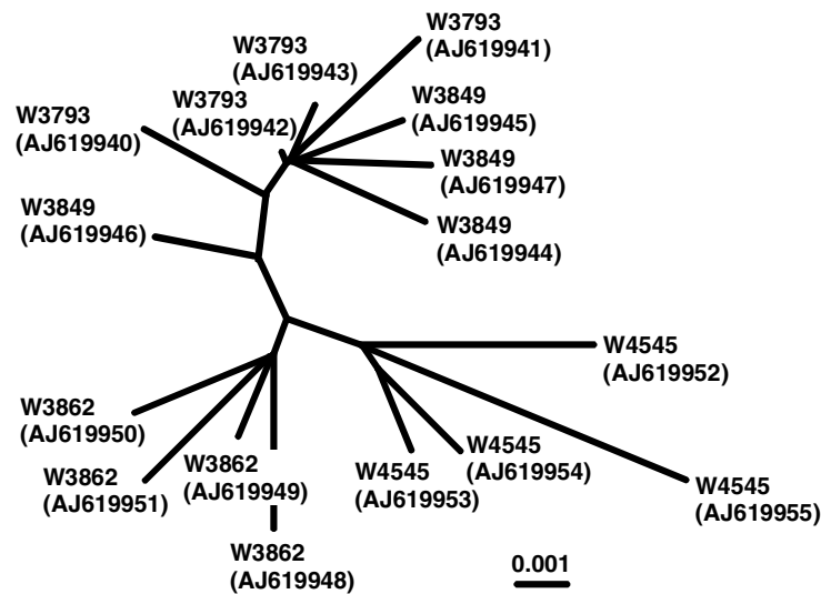
Fig. 2. ML analysis of the 16 Gerdemannia scintillans sequences, computed from 1722 aligned sites. Note that sequences from the spore from Poland (W3849) and those from Germany (W3793) form a mixed cluster.
