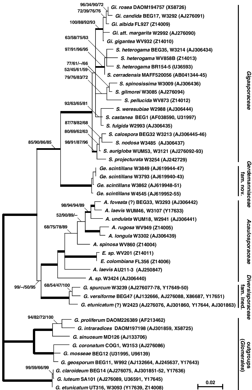
Fig. 1. Phylogenetic tree of the Diversisporales with members of the Glomerales ( Glomus groups Aa, Ab, B) as outgroups. Distances are derived from a ML analysis. The values given above the branches correspond to supports in NJ/MP/ML/ML-QP analyses. The thick lines represent branches which are supported by at least 95% in all analyses, the medium ones to branches supported by at least 85% in all analyses. Where no value is given, the topology is not reflected in the respective analysis. Topologies that are not supported by at least 50% in at least three of the analyses are collapsed to polytomies. A., Acaulospora ; E., Entrophospora ; Ge., Gerdemannia ; Gi., Gigaspora ; G., Glomus ; and S., Scutellospora .
